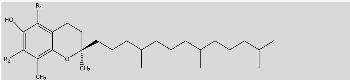
Figure 2 - Structure of tocopherols in Argan oil (R1 = R2 = CH 3 : \alpha - tocopherol; R1 = CH 3 , R2 = H: \beta - tocopherol; R1 = H; R2 = CH 3 : \gamma - tocopherol; R1 = R2 = H: \delta - tocopherol)
